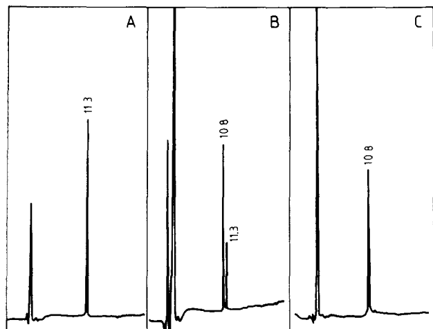
Fig. 2. Reverse-phase HPLC analysis of different stages of cyclic disulfide formation. (A) reduced, purified linear precursor, (B) after 24-h oxidation; and (C) fully oxidized, purified by gel permeation chromatography. HPLC conditions, see text.
